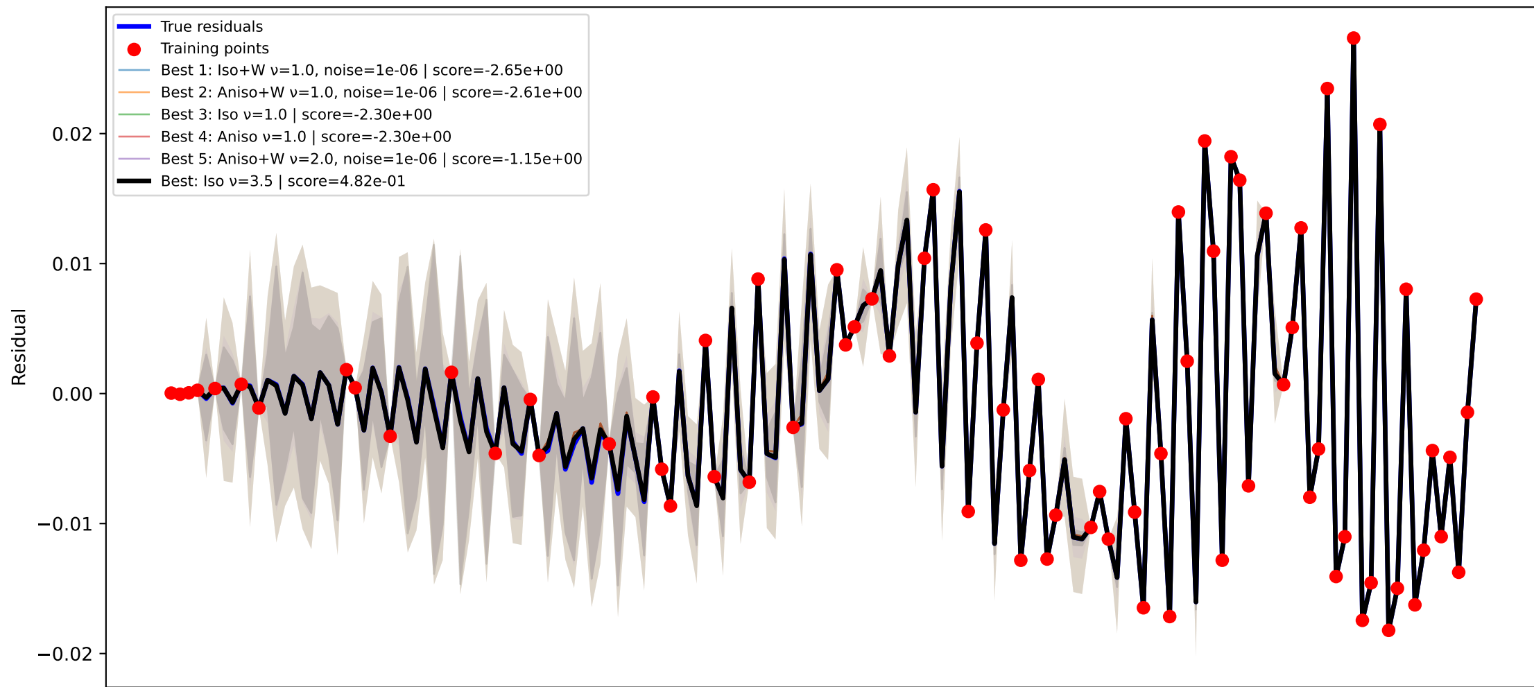
GPR kernel comparison node=32 RMSE=8.099e-05, train RMSE=1.419e-11
